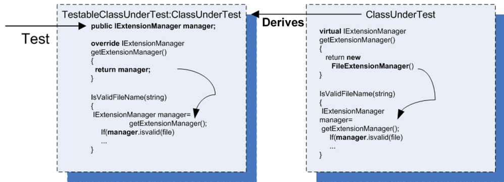
Figure 3.8 You inherit from the class under test so you can override its virtual factory method and return whatever object instance you want, as long as it implements IExtensionManager . Then you perform your tests against the newly derived class.
