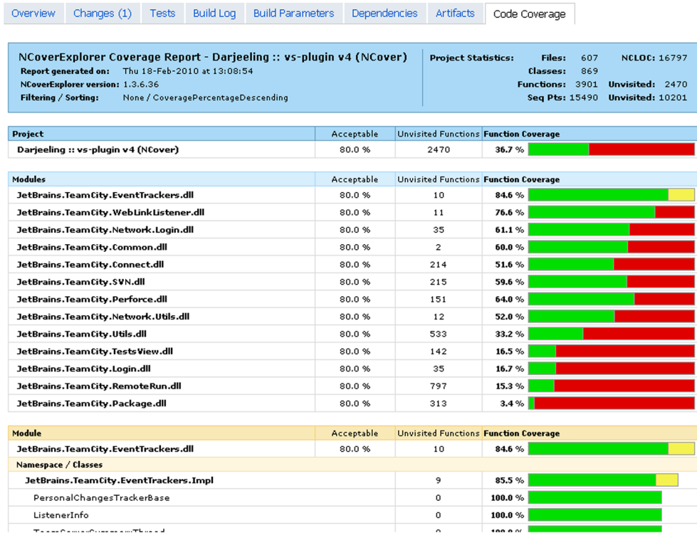
Figure 9.1 An example of a test-code-coverage report in TeamCity with NCover
