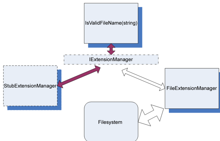
Figure 3.4 Introducing a stub to break the dependency. Now your class shouldn't know or care which implementation of an extension manager it's working with.
