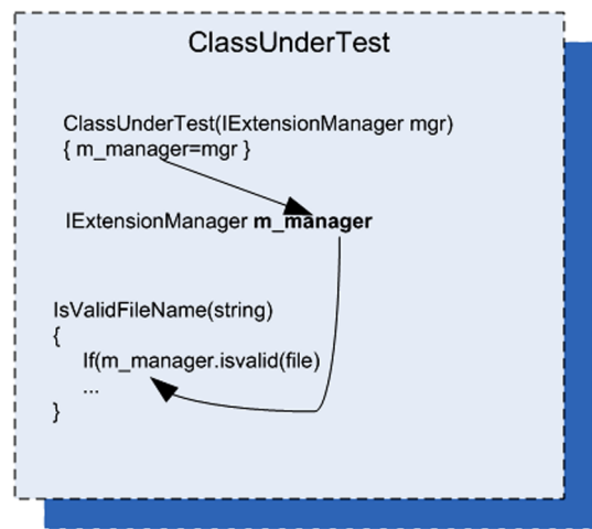
Figure 3.5 Flow of injection via a constructor
