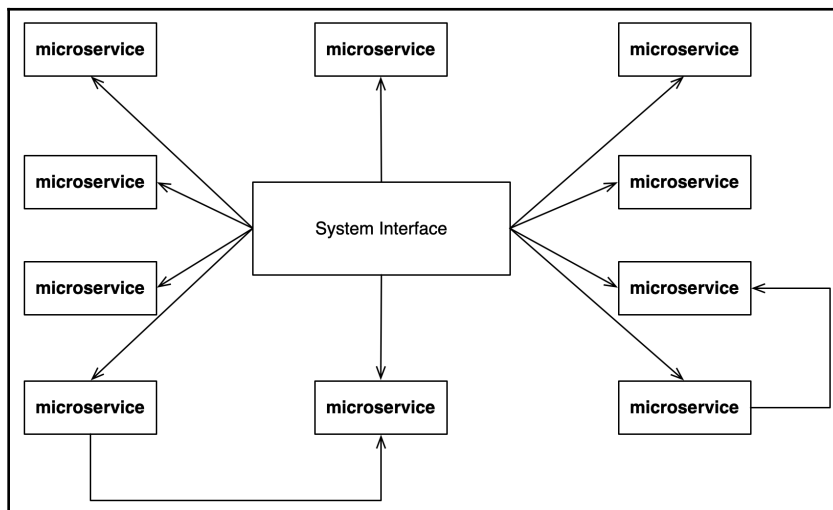
Microservices pattern
