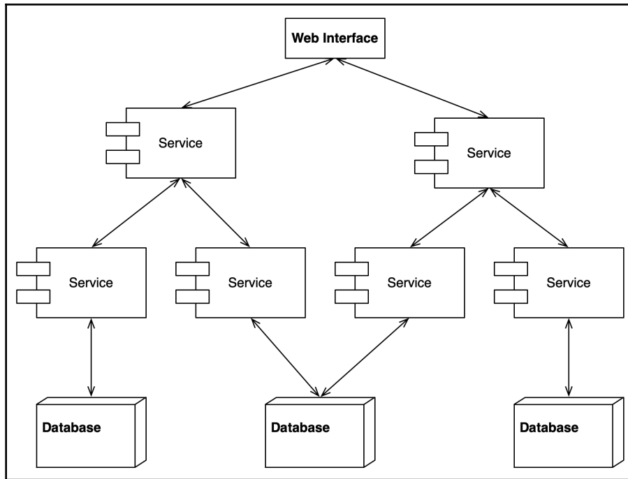
Service-oriented pattern—overview
