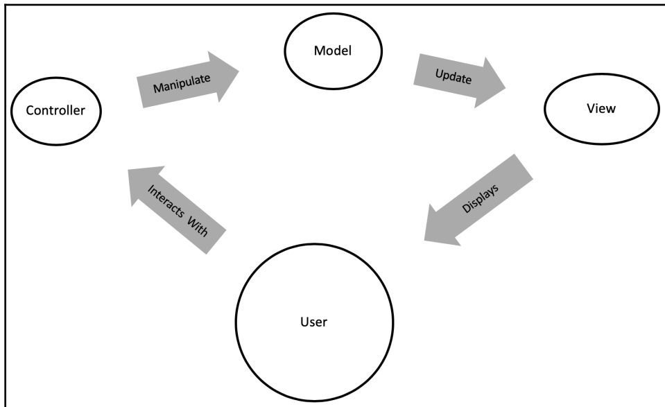
MVC pattern—overview
