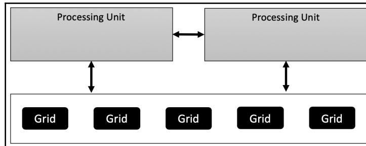
Space-based pattern—overview
