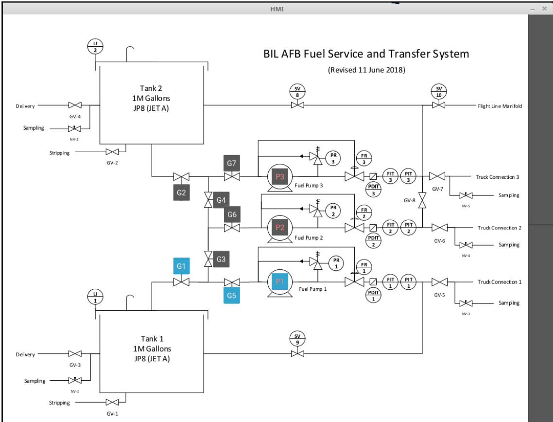
Tank 1-Pump1 drawing
