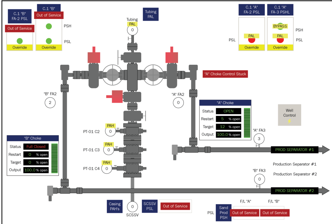
Example HMI
