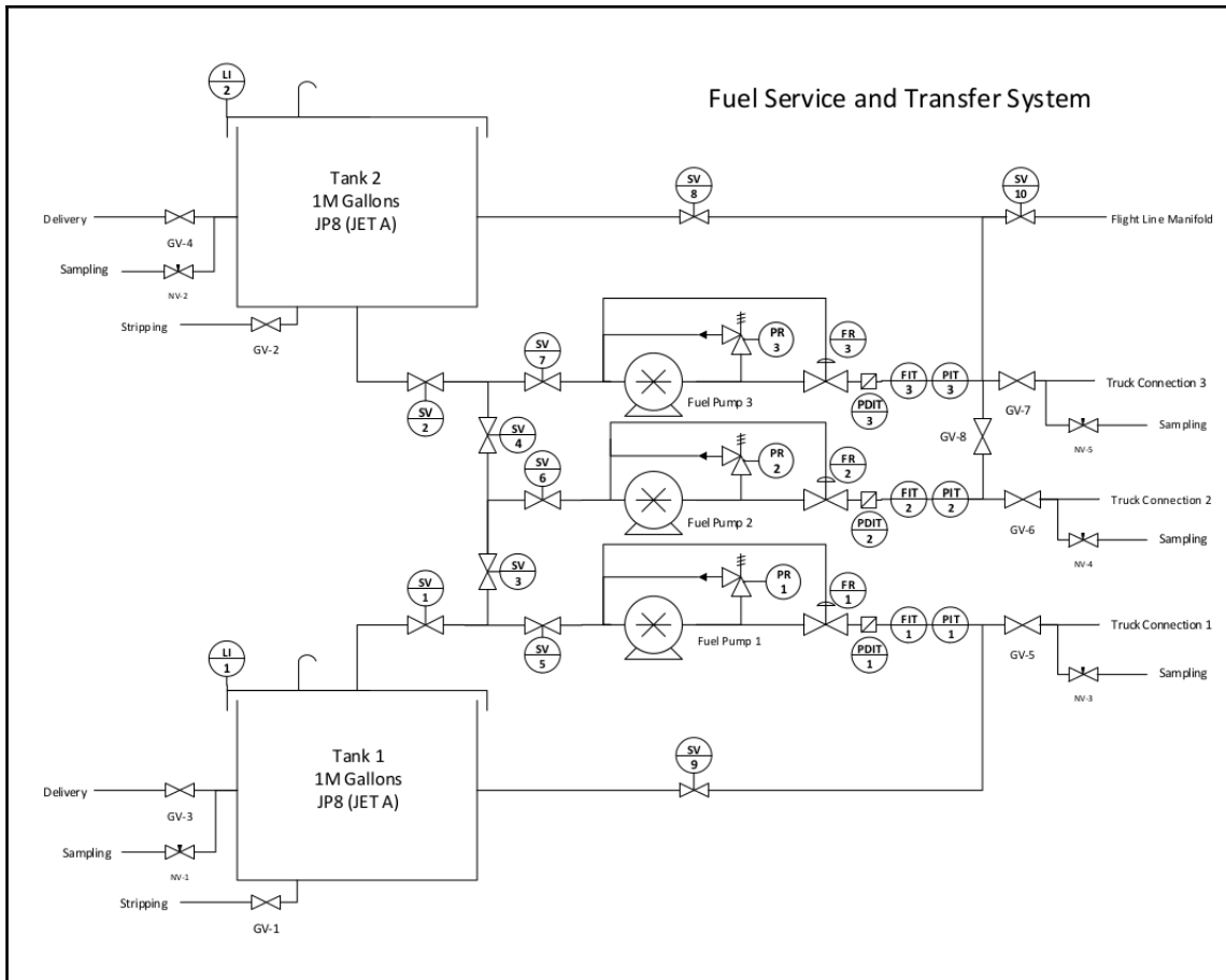
Fuel farm schematic
