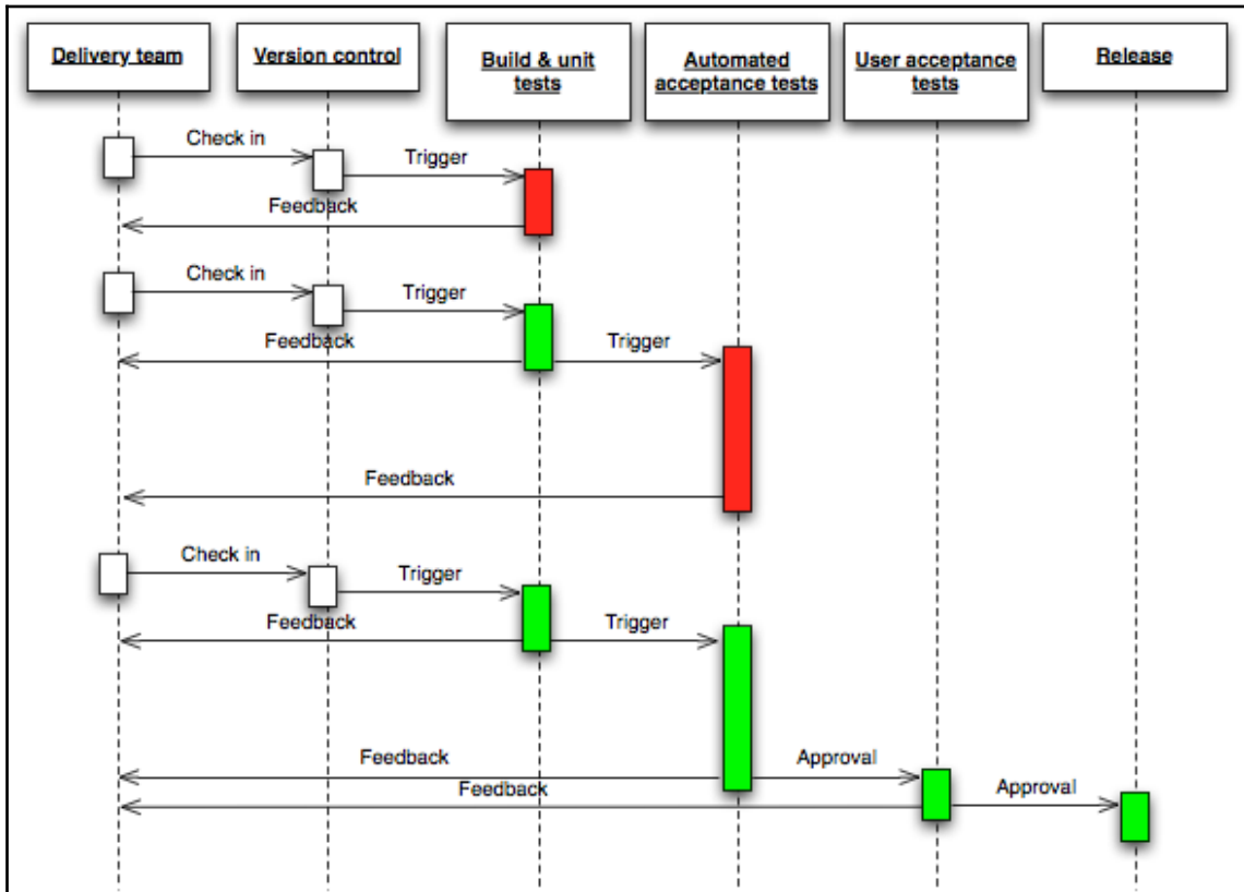
Continuous integration process
