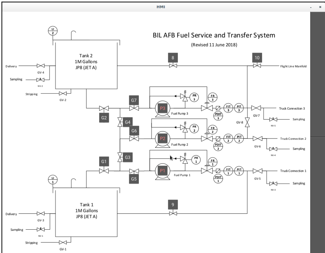
Kivy HMI (part 1)
