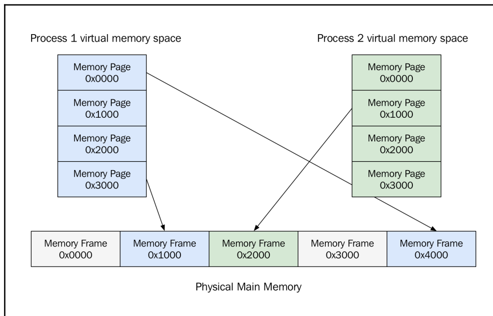
Virtual memory pages mapped to memory frames in physical memory. Virtual memory pages that are not in use do not have to occupy physical memory.
