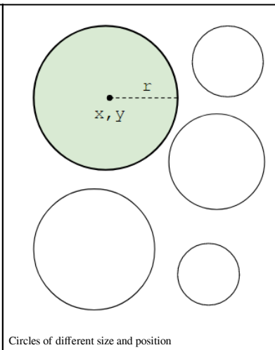
Circles of different size and position
