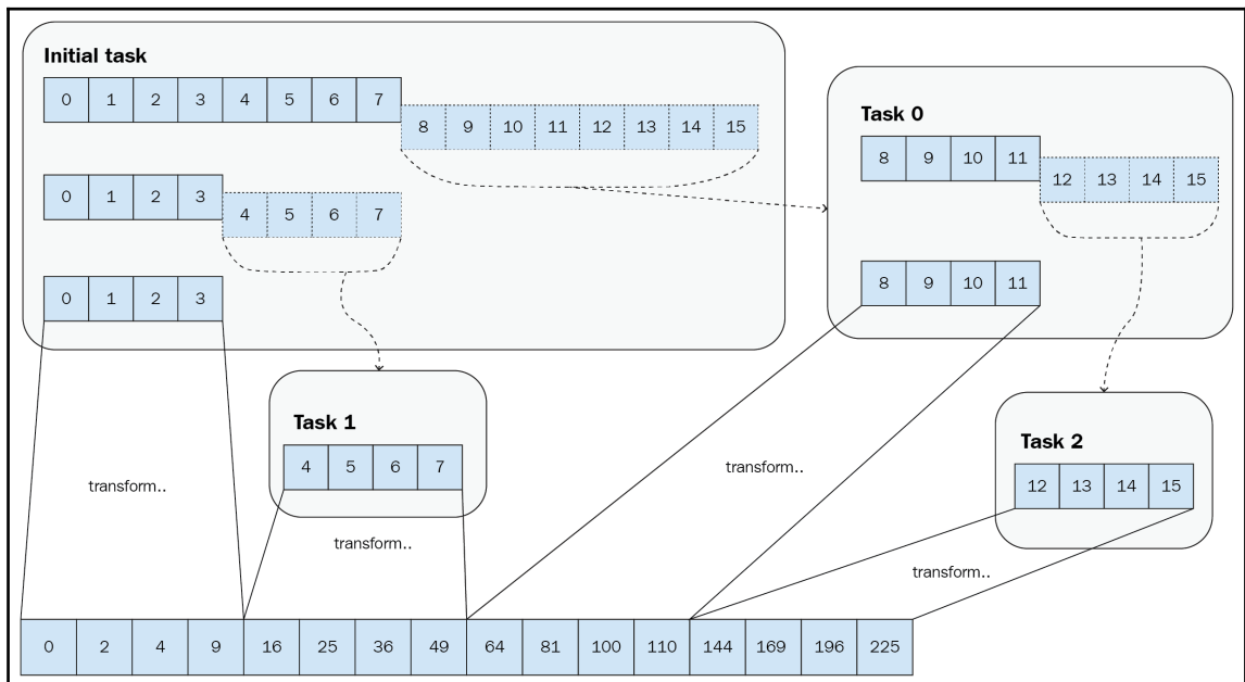
A range is divided recursively for parallel processing
