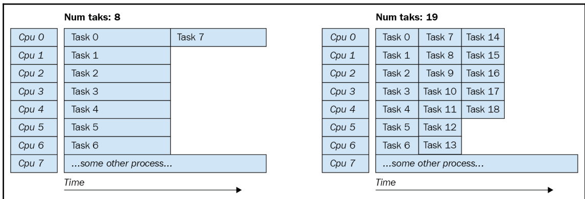
Possible scenarios where computation time is proportional to chunk size
