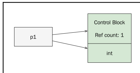
A shared_ptr instance p1 which points to the integer object and a control block which contains the reference counting. In this case, there is only one shared pointer using the int , and hence the ref count is 1.
