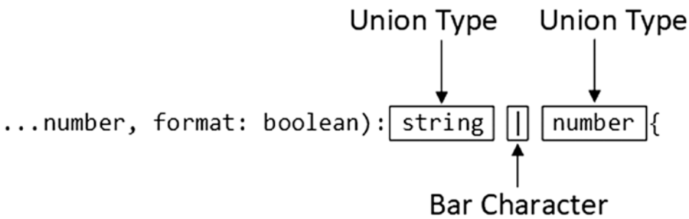
Figure 7-2. Defining a type union
