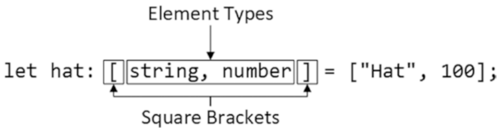
Figure 9-2. Defining a tuple
