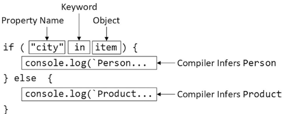
Figure 10-4. Using the in keyword
