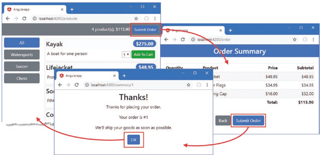
Figure 18-2. Adding components to the example application
