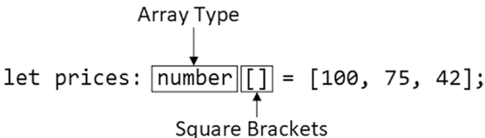
Figure 9-1. An array type annotation
