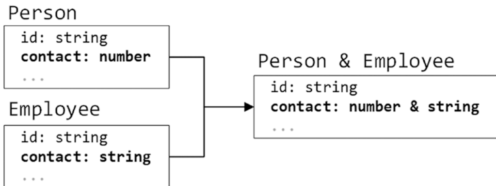
Figure 10-9. Merging properties with different types
