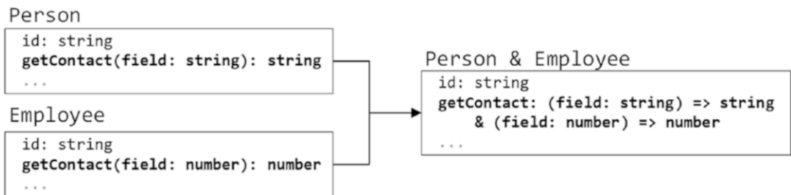
Figure 10-11 Merging methods
