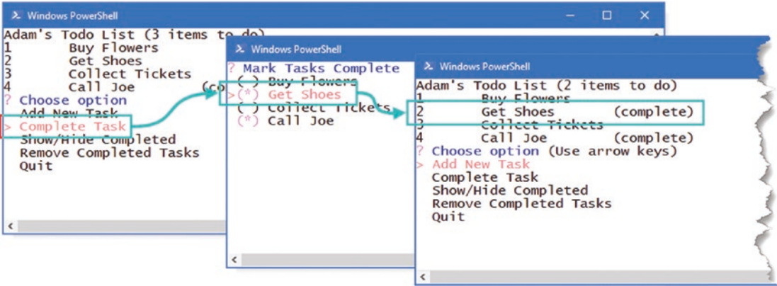
Figure 1-5. Completing items
