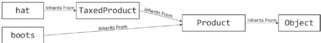
Figure 4-4. A more complex prototype chain
