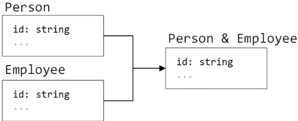
Figure 10-8. Merging properties with the same type
