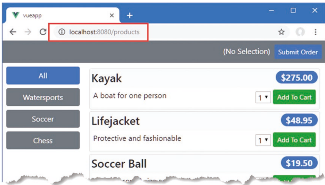
Figure 22-2. Using URL routing
