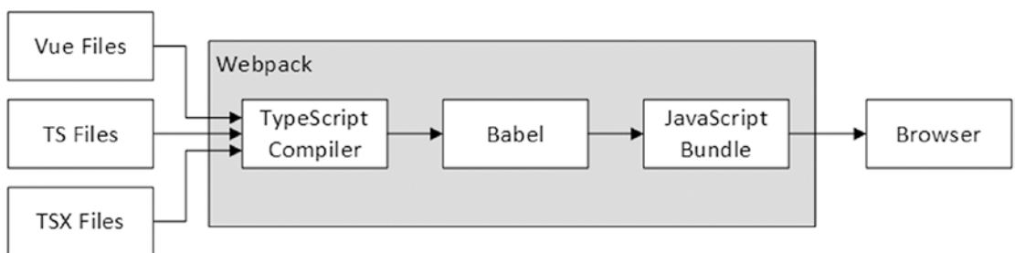
Figure 21-2. The Vue.js toolchain
