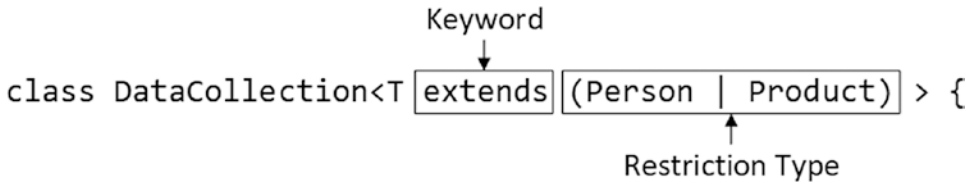
Figure 12-3. A generic type parameter restriction
