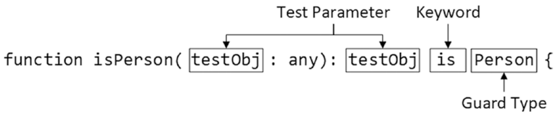
Figure 10-5. An object type guard function
