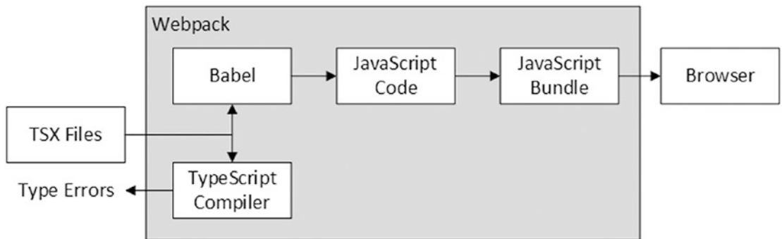
Figure 19-3. The TypeScript React development toolchain
