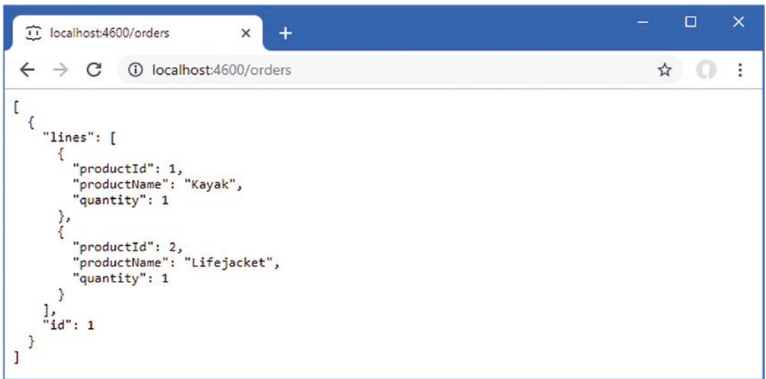
Figure 16-7. Inspecting the submitted orders
