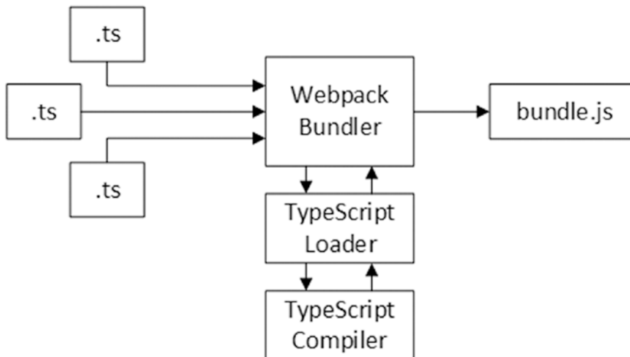
Figure 15-2. Adding a bundle to the toolchain
