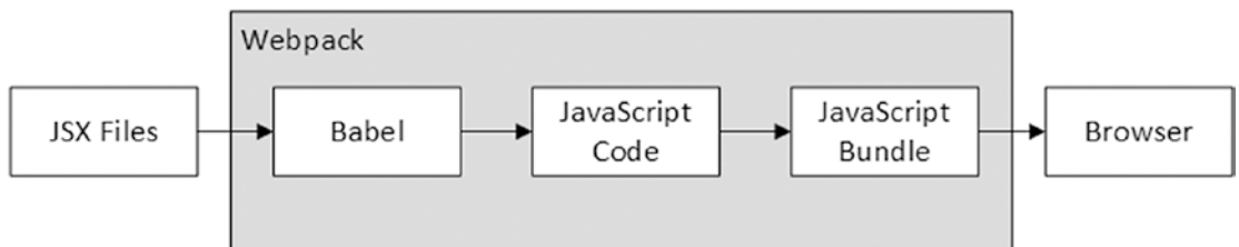
Figure 19-2. The JavaScript React development toolchain
