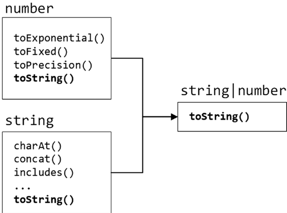
Figure 7-3 The effect of a type union
