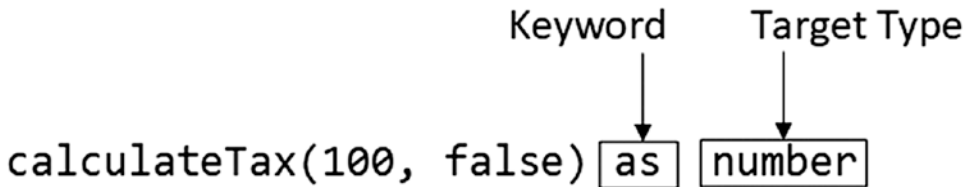
Figure 7-4. Asserting a type
