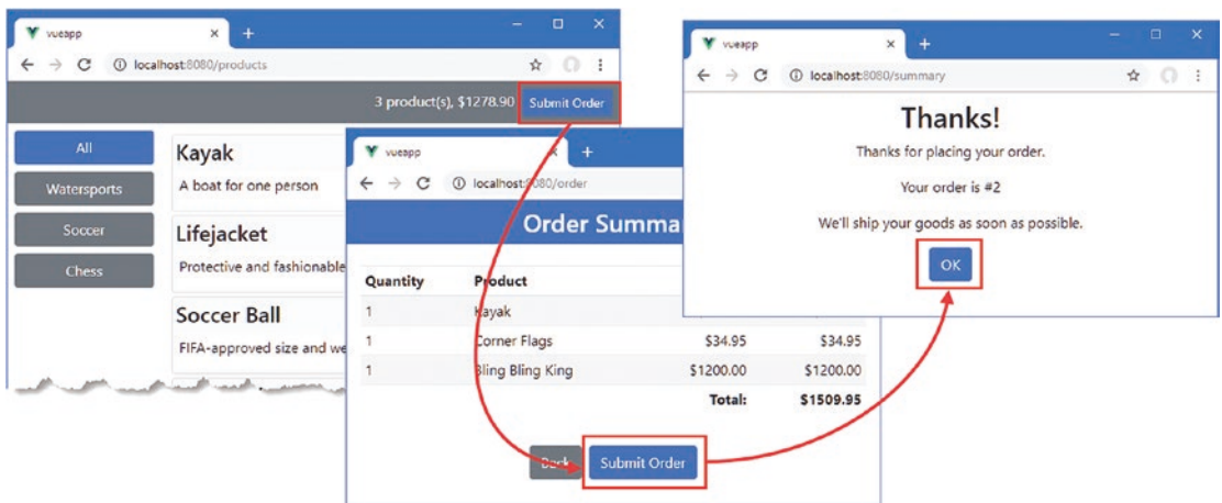
Figure 22-3. Completing the example application
