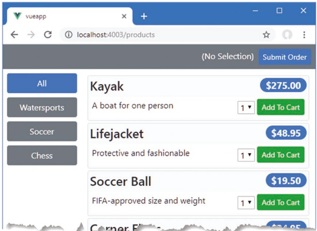
Figure 22-5. Running the containerized application
