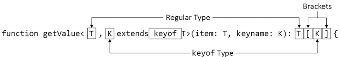
Figure 13-2. The indexed access operator
