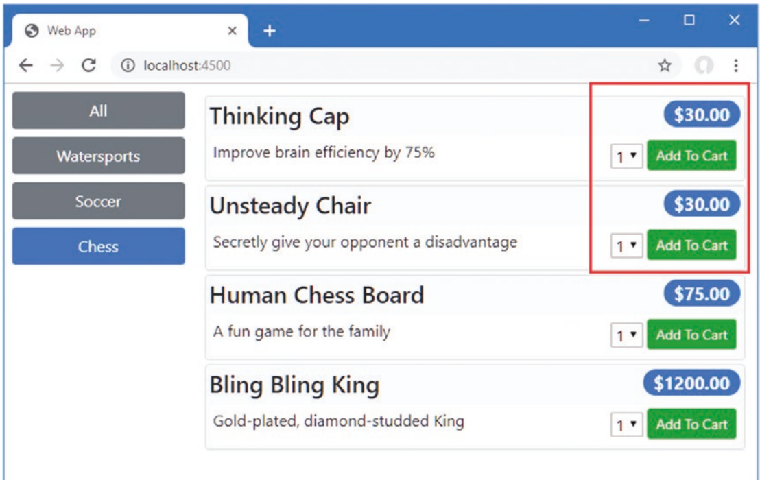
Figure 16-4. Using a decorator to enforce a minimum value
