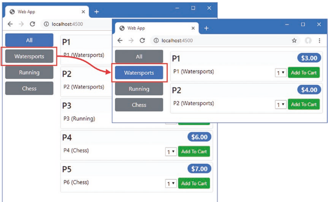
Figure 15-8. Displaying products
