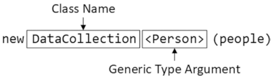
Figure 12-2. Creating an object with a generic type argument
