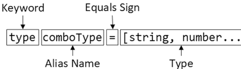
Figure 9-5. Defining a type alias
