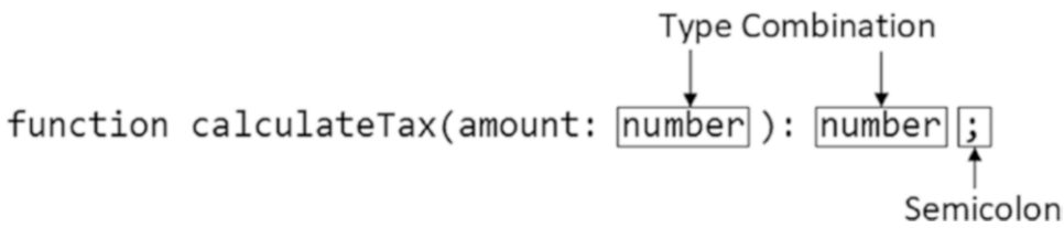
Figure 8-4. A function type overload
