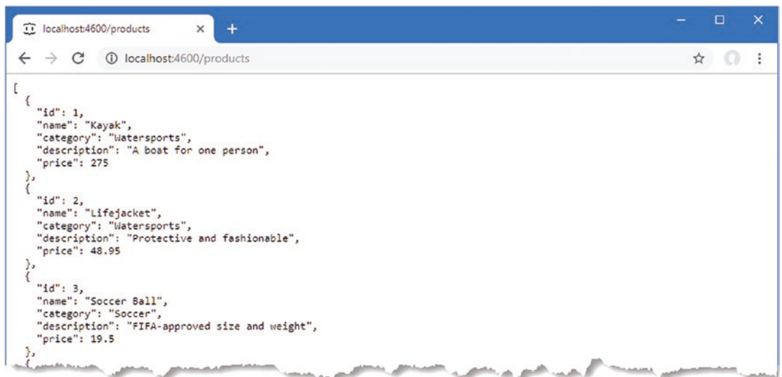
Figure 16-1. Getting data from the web service
