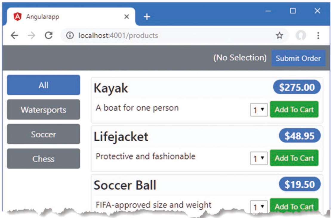
Figure 18-3. Running the production build
