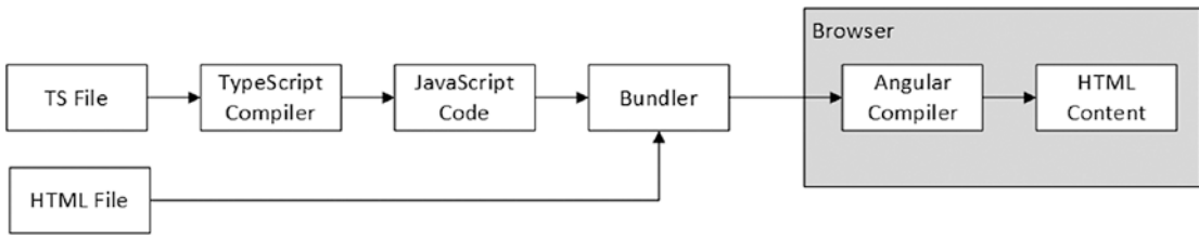
Figure 17-3. The two Angular compilation stages
