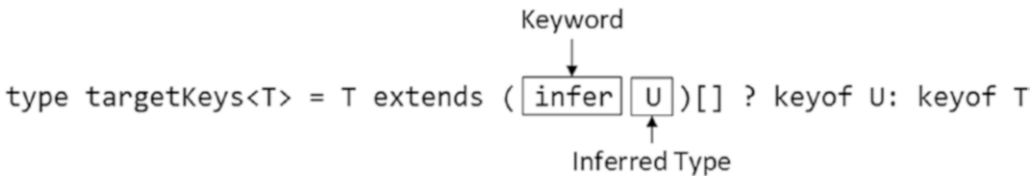
Figure 13-5. Inferring a type in a conditional type
