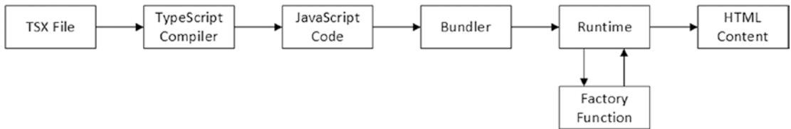
Figure 15-6. Transforming JSX
