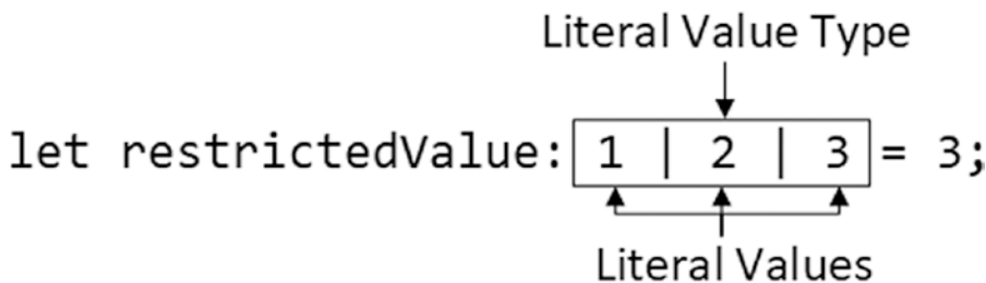
Figure 9-4. A literal value type
