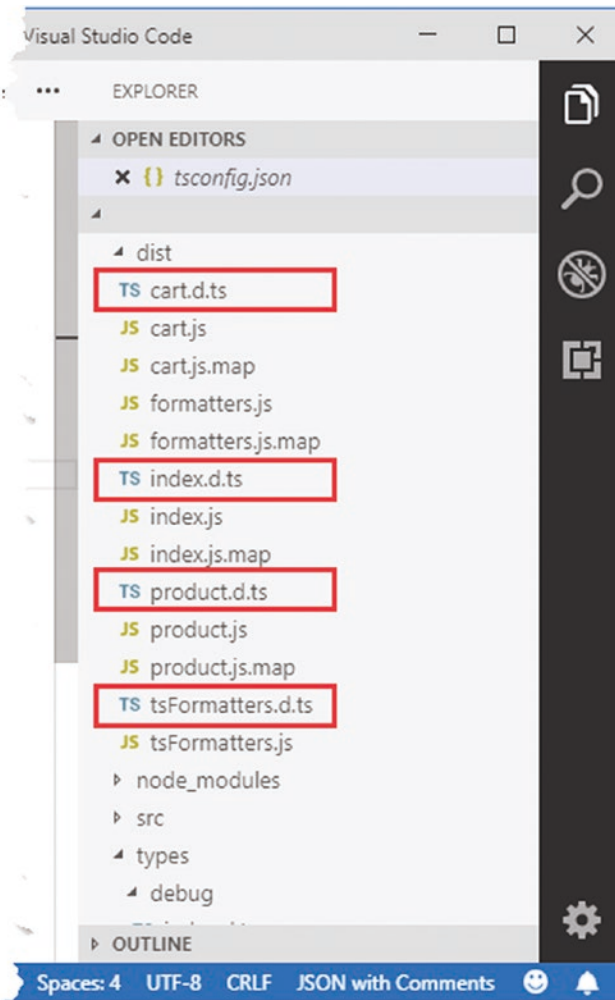
Figure 14-2. Generating declaration files
