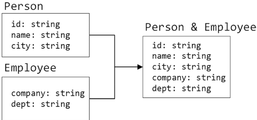
Figure 10-7. The effect of a type intersection
