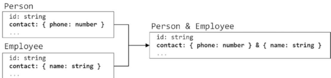
Figure 10-10. Merging properties with shape types
