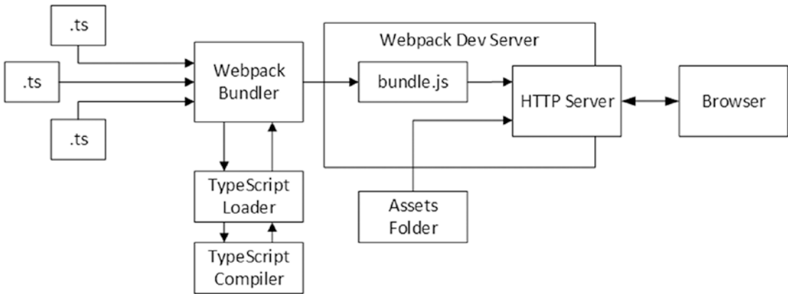
Figure 15-4. Adding WDS to the development toolchain
