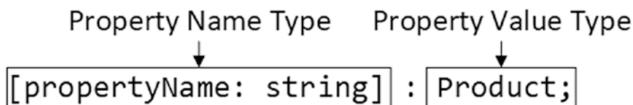
Figure 11-9. An index signature
